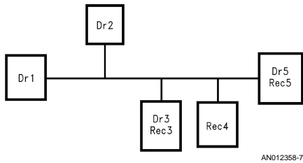
FIGURE 7. Bus Topology
