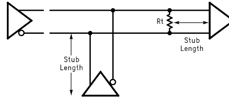
FIGURE 9. Stub Length
